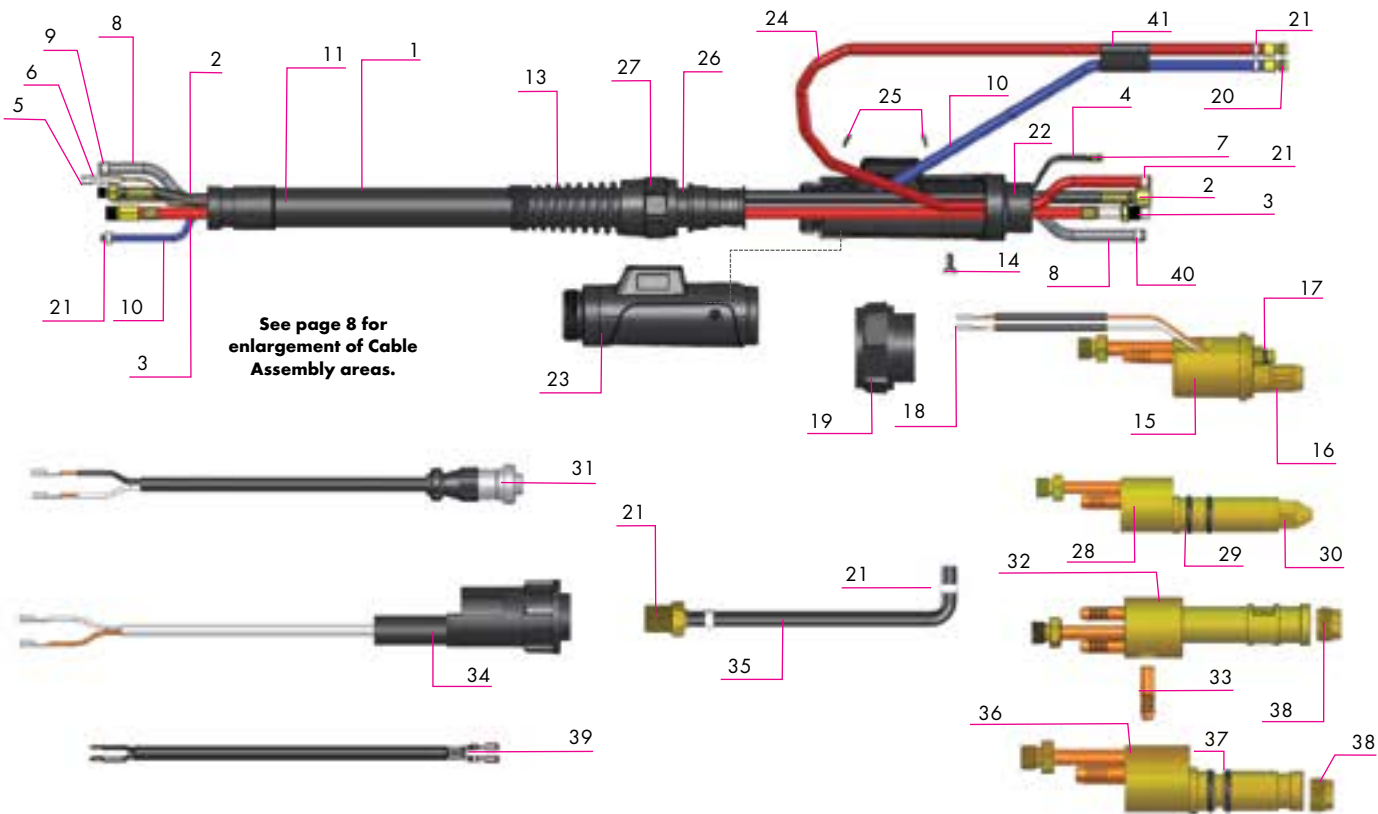
MB 501D Body Cable Assembly
